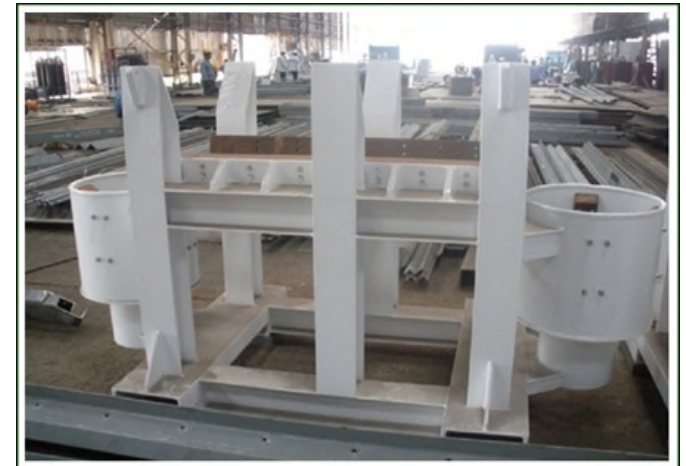
CRANE BLOCK STORAGE FRAME
